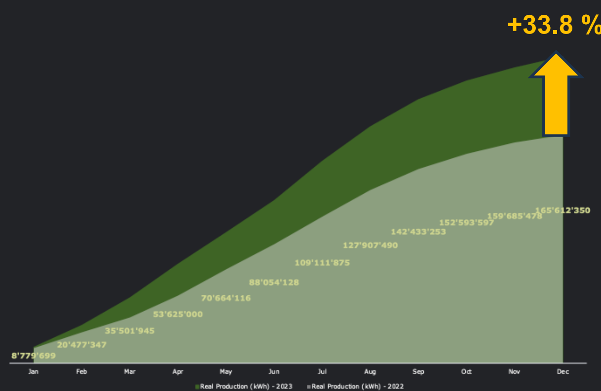
Accumulated Production (kWh)
