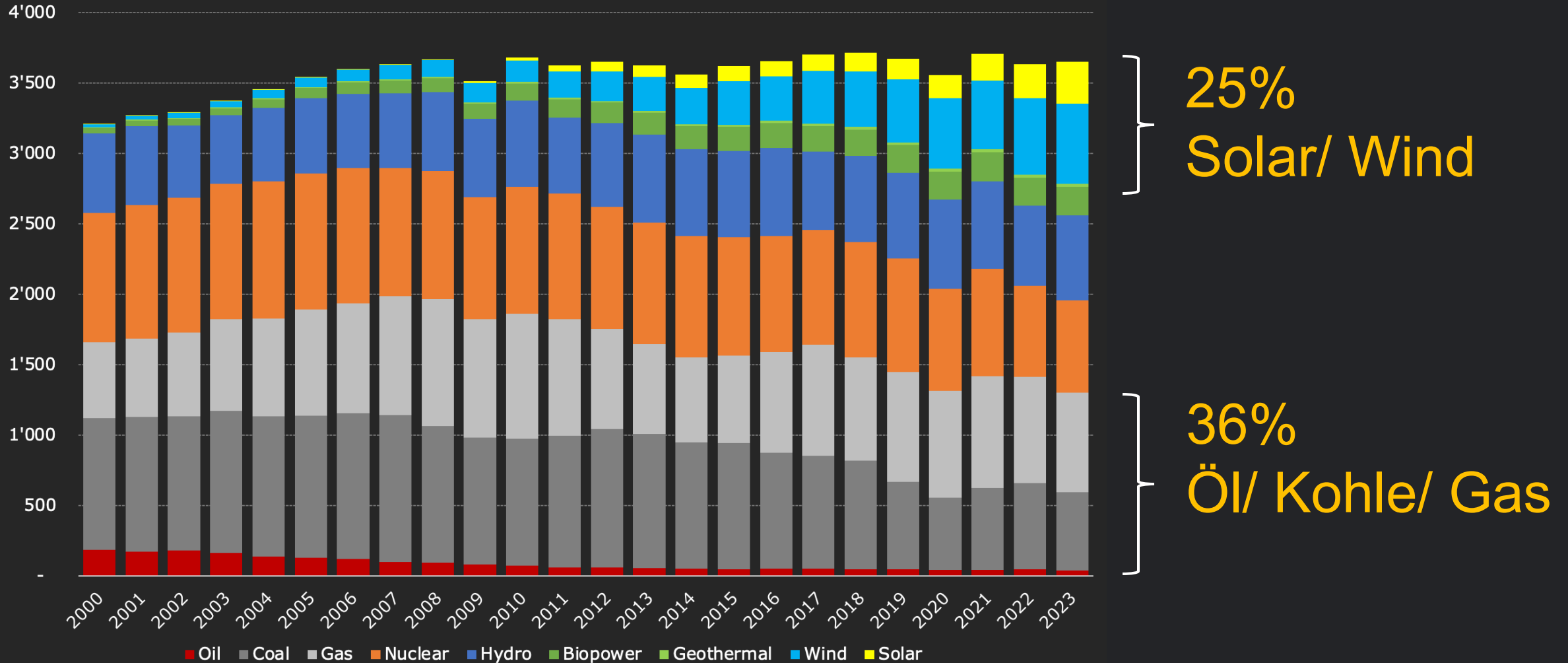
Electricity production in Western Europe (TWh)
